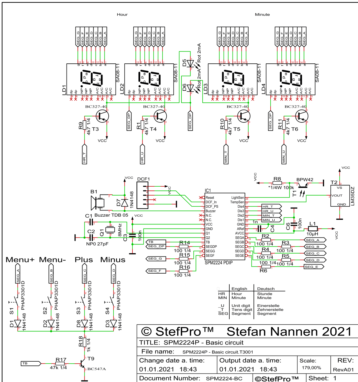
Figure 2: Basic circuit of SPM2224P
