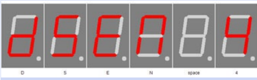
DCF sensitivity
