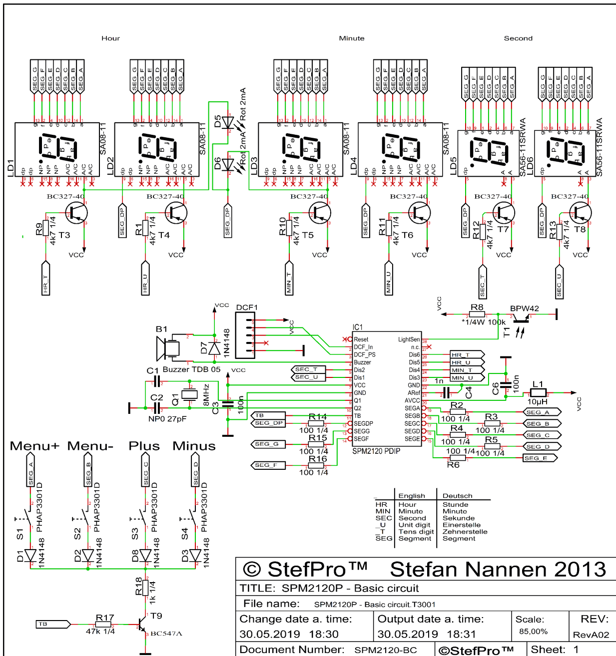
Figure 2: Basic circuit of SPM2220P
