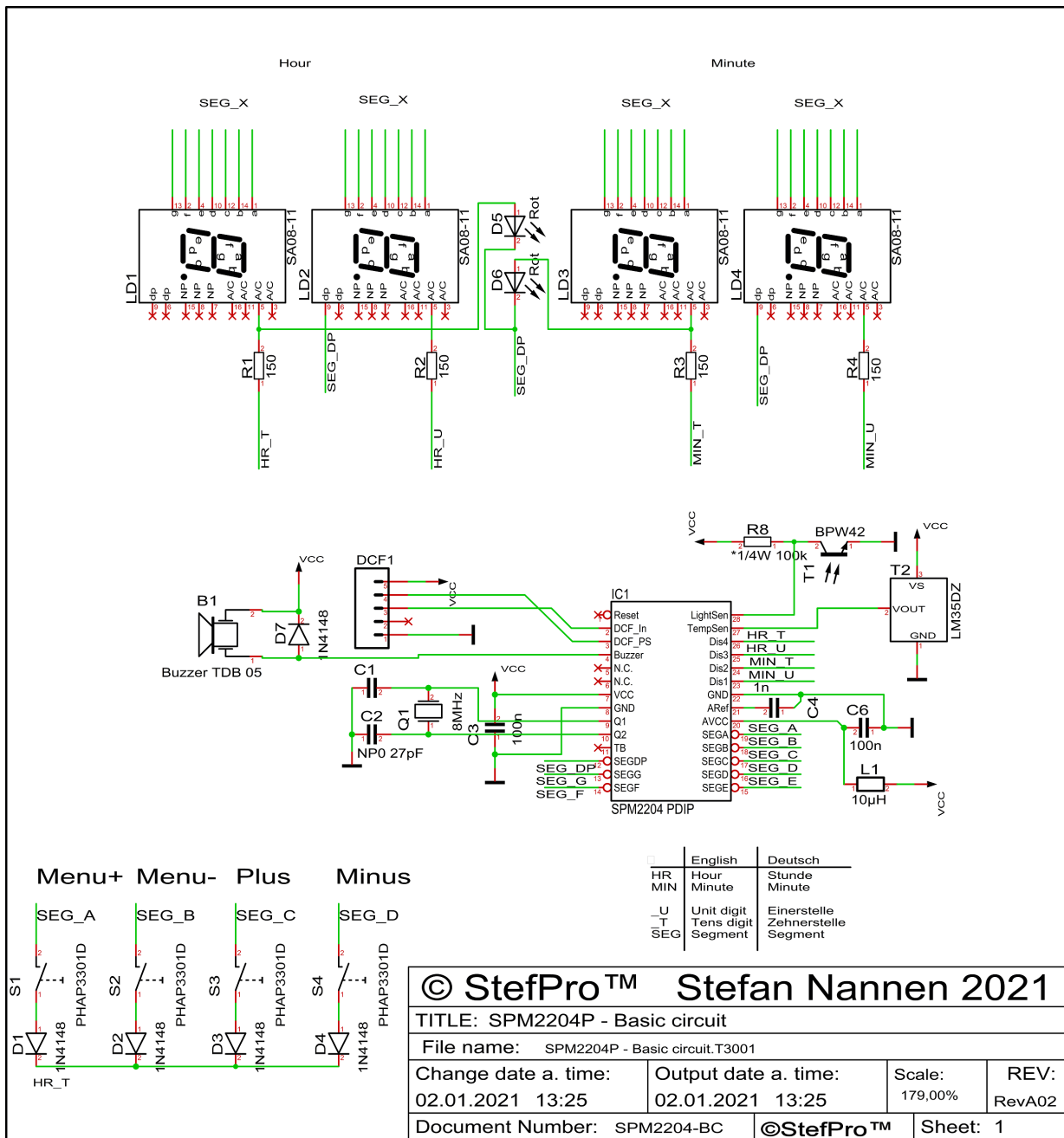
Figure 2: Basic circuit of SPM2204P
