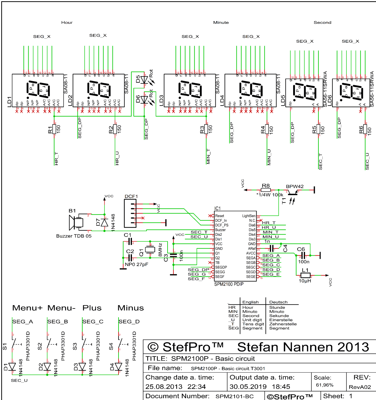
Figure 2: Basic circuit of SPM2200P
