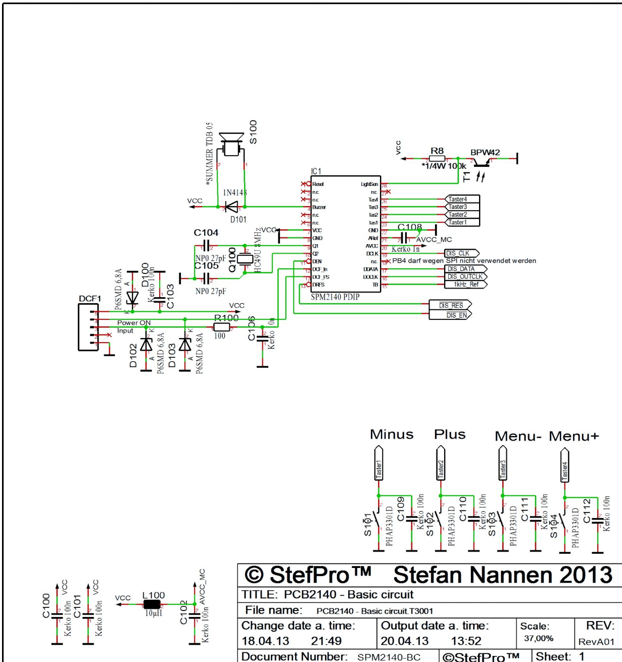
Figure 2: Basic circuit of SPM2140P part 1
