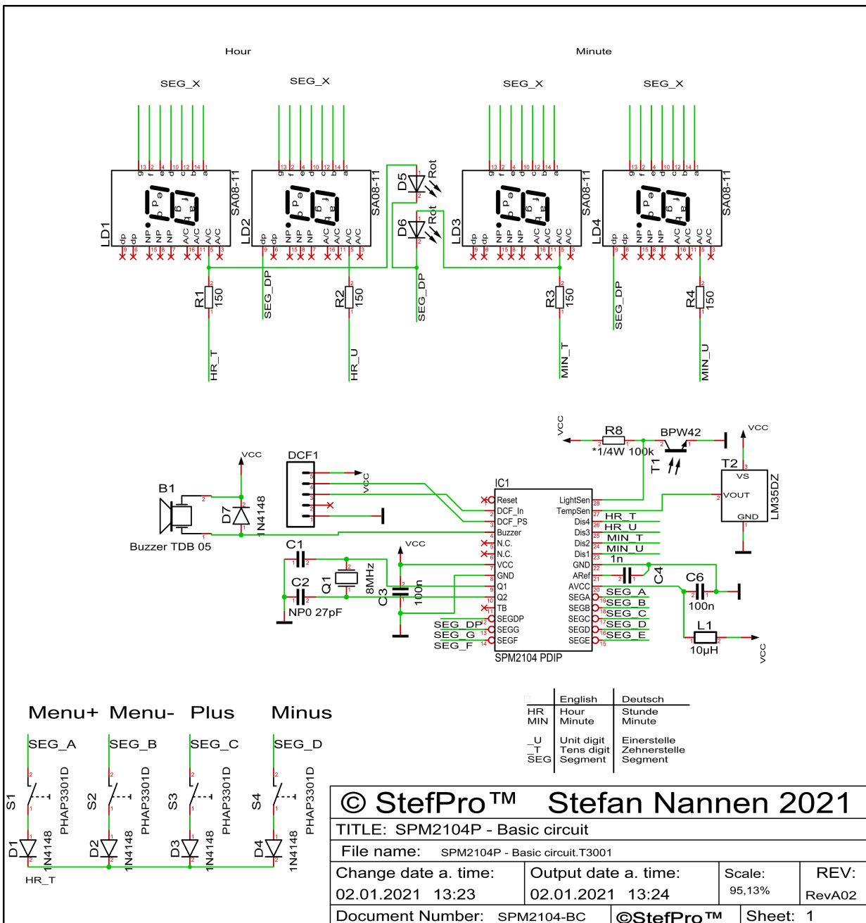
Figure 2: Basic circuit of SPM2104P
