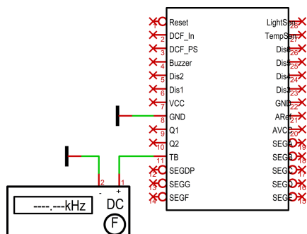
Figure 12: Calibrate quartz
