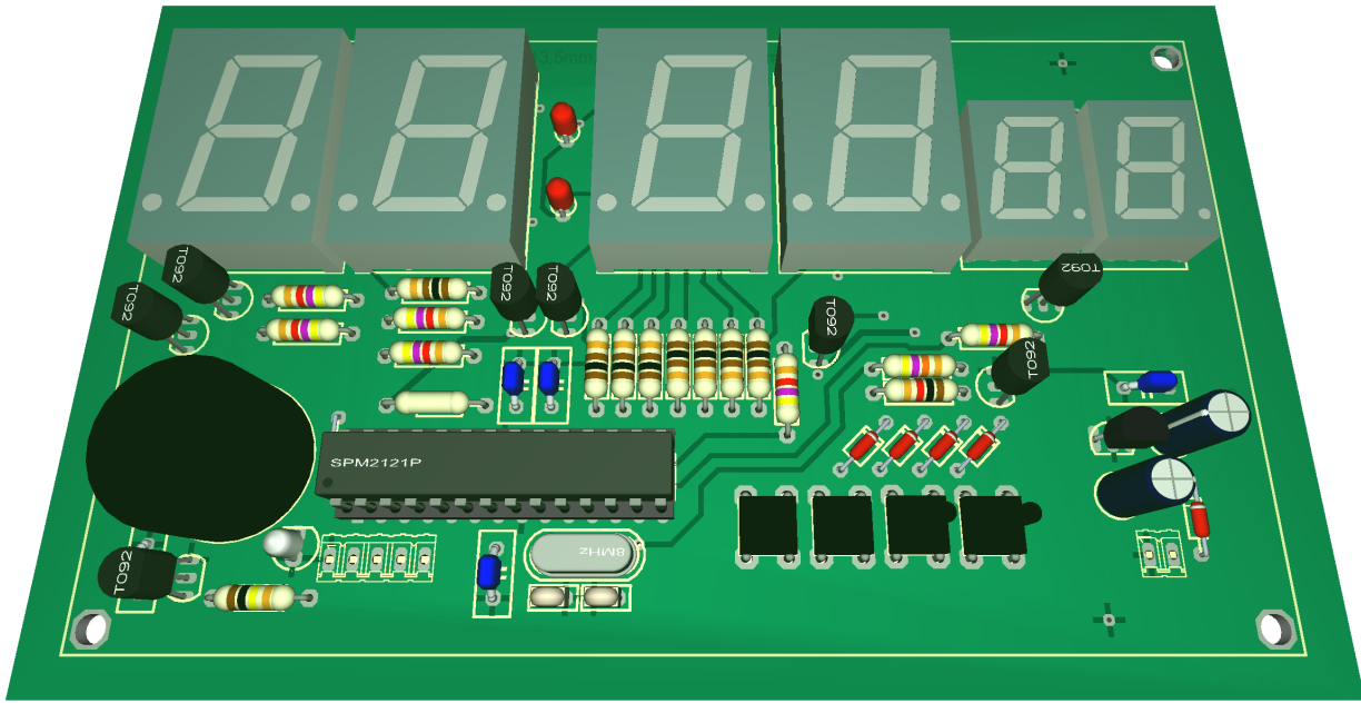
Figure 11: Basic assembly of SPK2121.01 step 7 The finally assembled pcb, only the wires for the supply voltage and the DCF receiver are missing.
