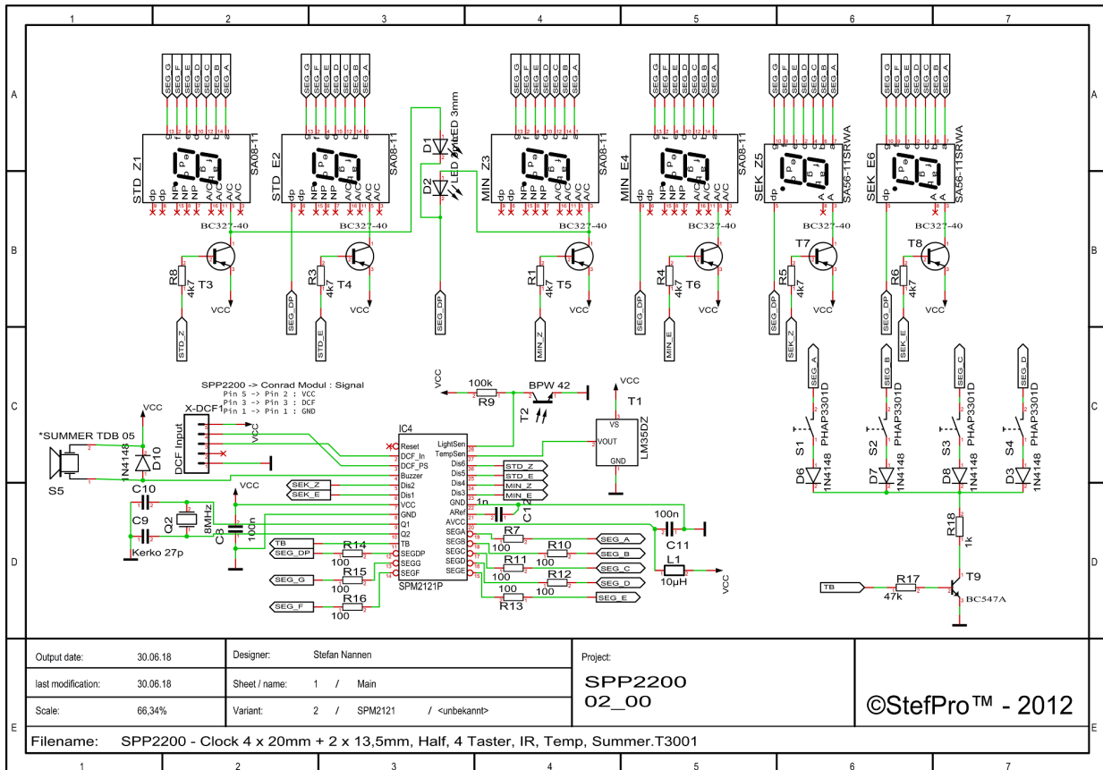
Figure 1: Basic circuit of SPK2121.01 part 1
