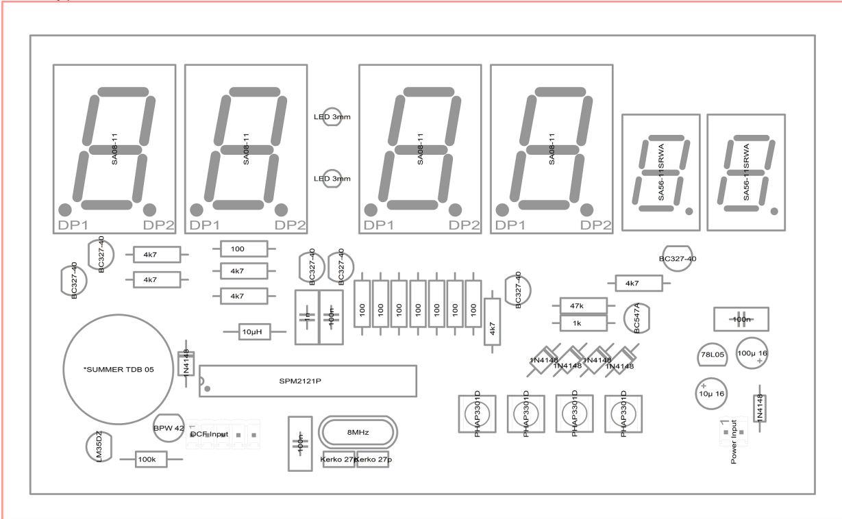
Figure 4: Basic assembly of SPK2121.01 1 Assembly plan with values
