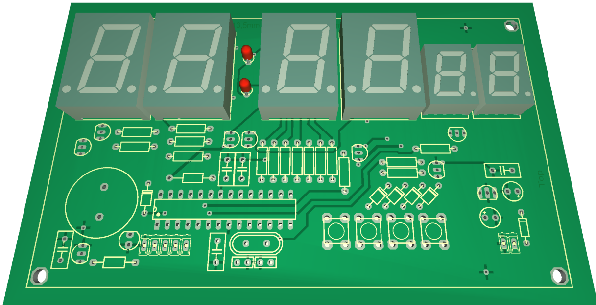
Figure 10: Basic assembly of SPK2121.01 step 6 Finally, the LEDs and 7 segment displays (these are to be ordered separately), these are to be soldered directly onto the PCB.
