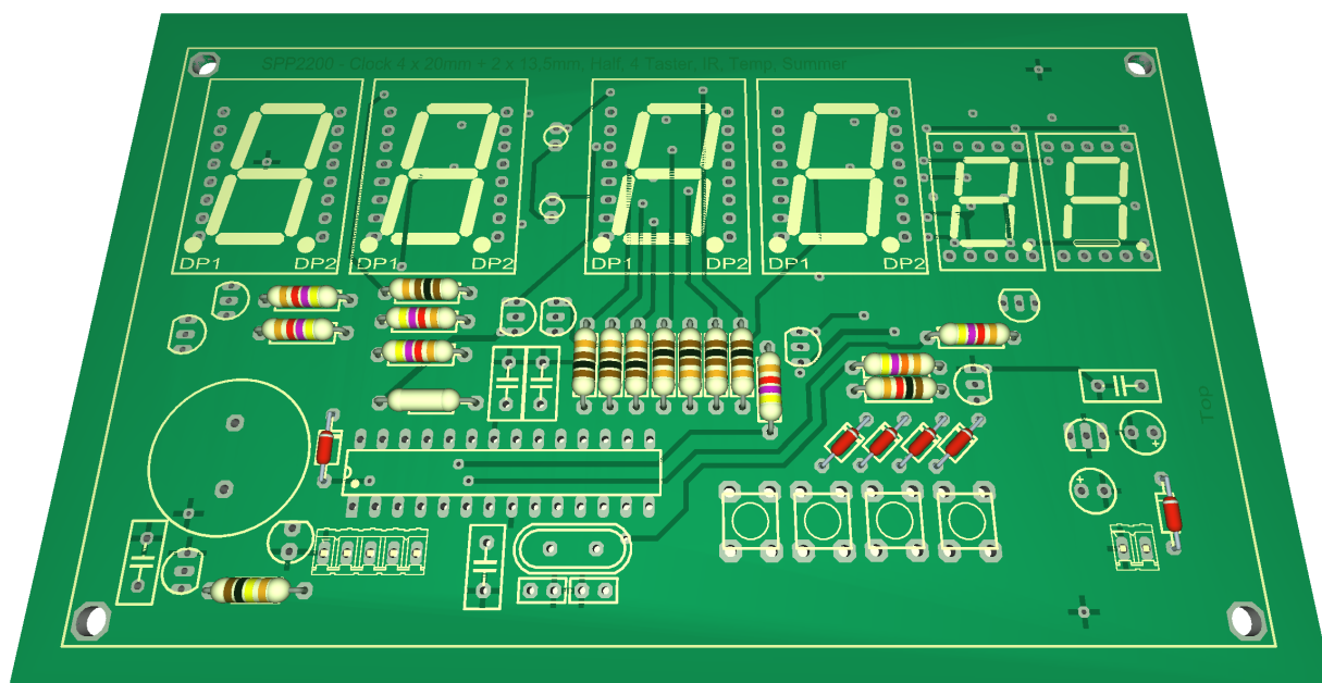
Figure 5: Basic assembly of SPK2121.01 step 1
