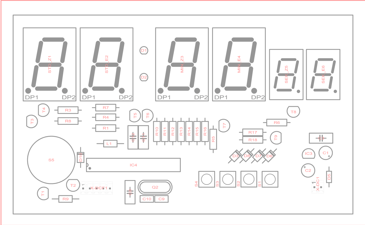
Figure 3: Basic assembly of SPK2121.01 Assembly plan with names
